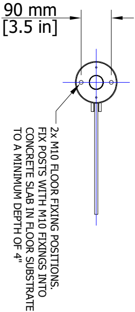
1500 HEIGHT INFILL
