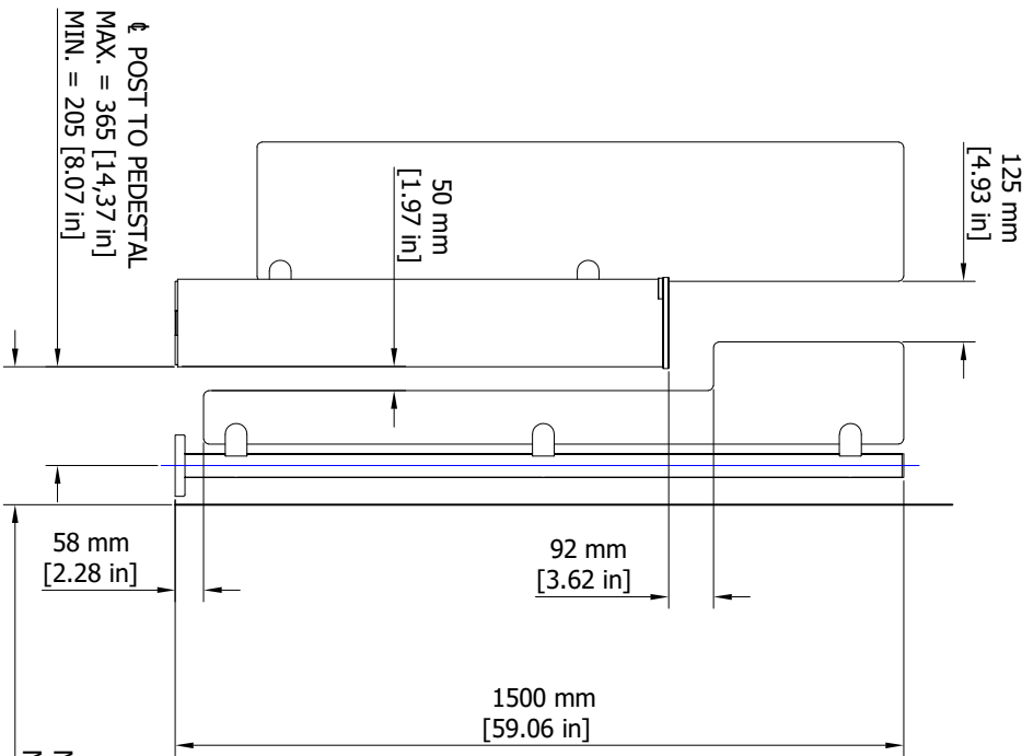
1500 HEIGHT GG250 PLUS HANGING INFILL
